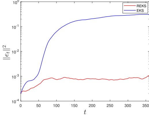
Fig. 1: Average variance of the estimation error for EKS and REKS with L = 40 in Case 1.
