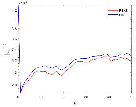
Fig. 2: Average variance of the estimation error for REKS and EKS with L = 10 in Case 2.
