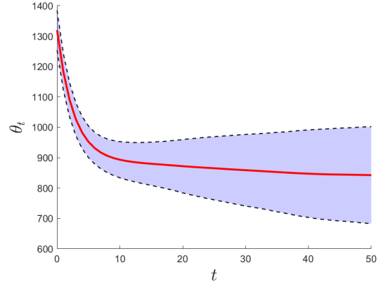
Fig. 3: Distribution over 2000 trials for the risk sensitivity parameter \theta_t of REKS with c_t = 10^{-2} in Case 2: the red line denotes its profile on average while the dashed lines define the corresponding confidence intervals (with level 0.95).
